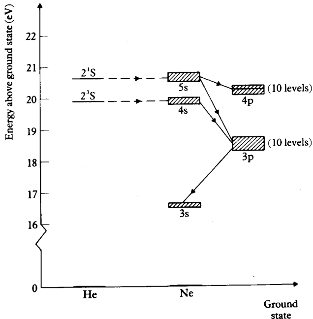
14.6 The energy levels of the He-Ne laser. The neon configuration concerned is (1s)^2(2s)^2(2p)^5 nl ; each configuration giving rise to a number of levels within the shaded regions. Note that in many textbooks, the (3s), (4s) and (5s) level are labelled (1s), (2s) and (3s), while the (3p) and (4p) levels are labelled (2p) and (3p). This alternative notation is due to Paschen.
